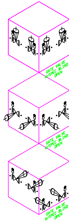
GATE VALVE W/SPEC BLIND OPEN
