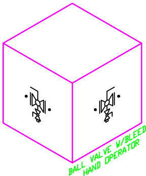
BALL VALVE W/ BLEED
