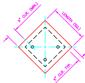
SEC. A SUPPORT REBAR
