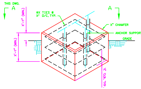
DET. 2 SUPPORT REBAR
